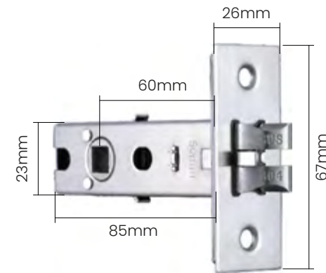
60 Single Latch (Center distance 60mm)
