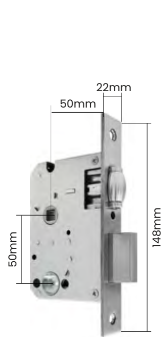
5050 Roller Latch Mortise
