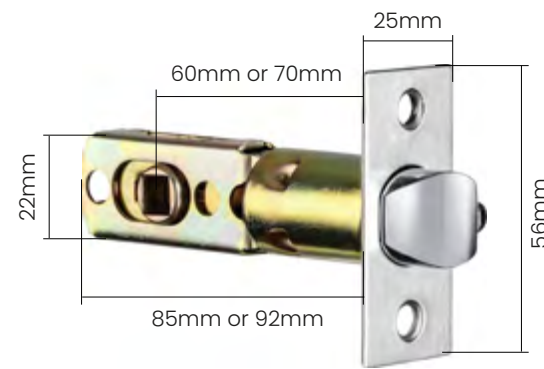
Adjustable Single Latch (Center distance 60 or 70mm)
