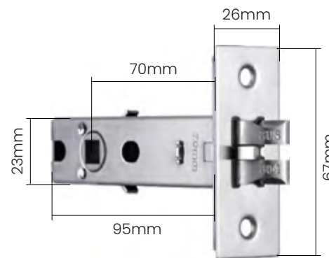
70 Single Latch (Center distance 70mm)
