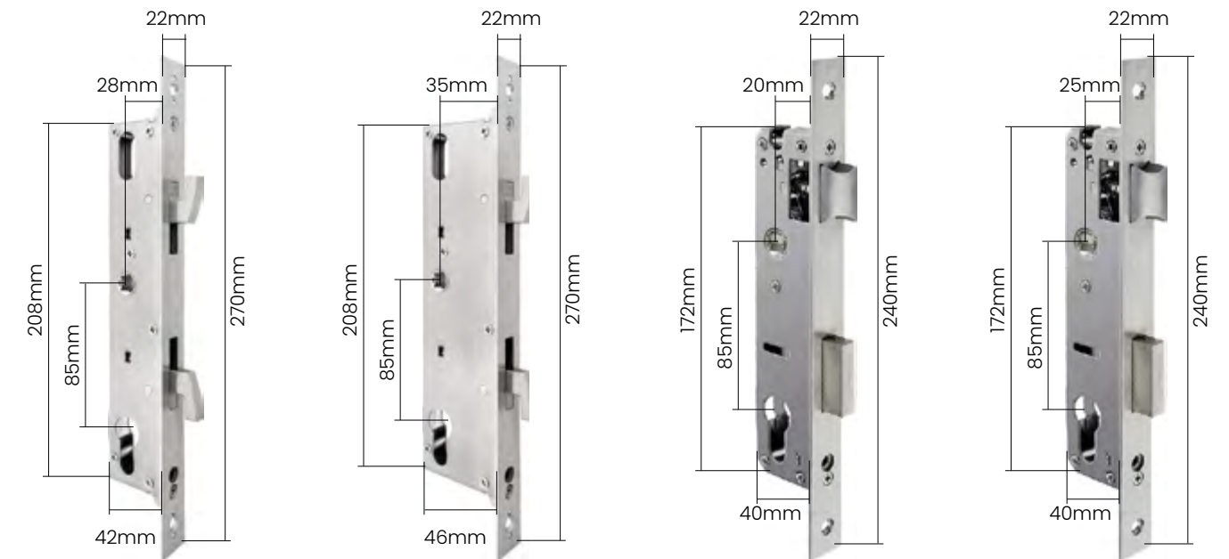
2885 (22×270mm) Sliding Mortise
