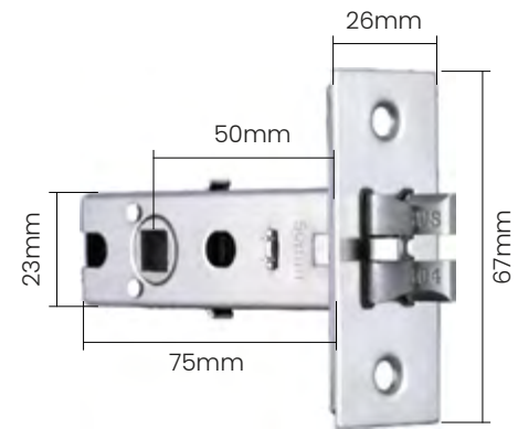
50 Single Latch (Center distance 50mm)
