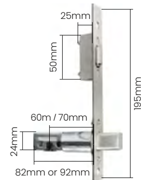
Roller Latch Deadbolt (Center distance 60 or 70mm)
